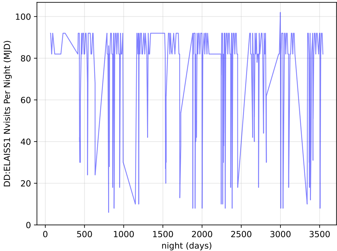
too_elab_r64_d3_griz_v3.4_10yrs all bands: DD:ELAISS1 Nvisits Per Night
