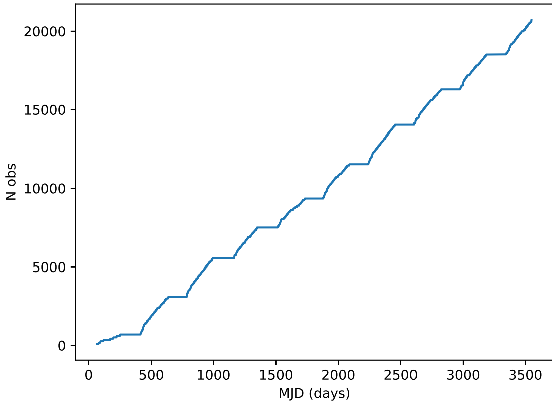
too_elab_r64_d3_griz_v3.4_10yrs all bands: DD:ELAISS1 Cumulative NVisits
