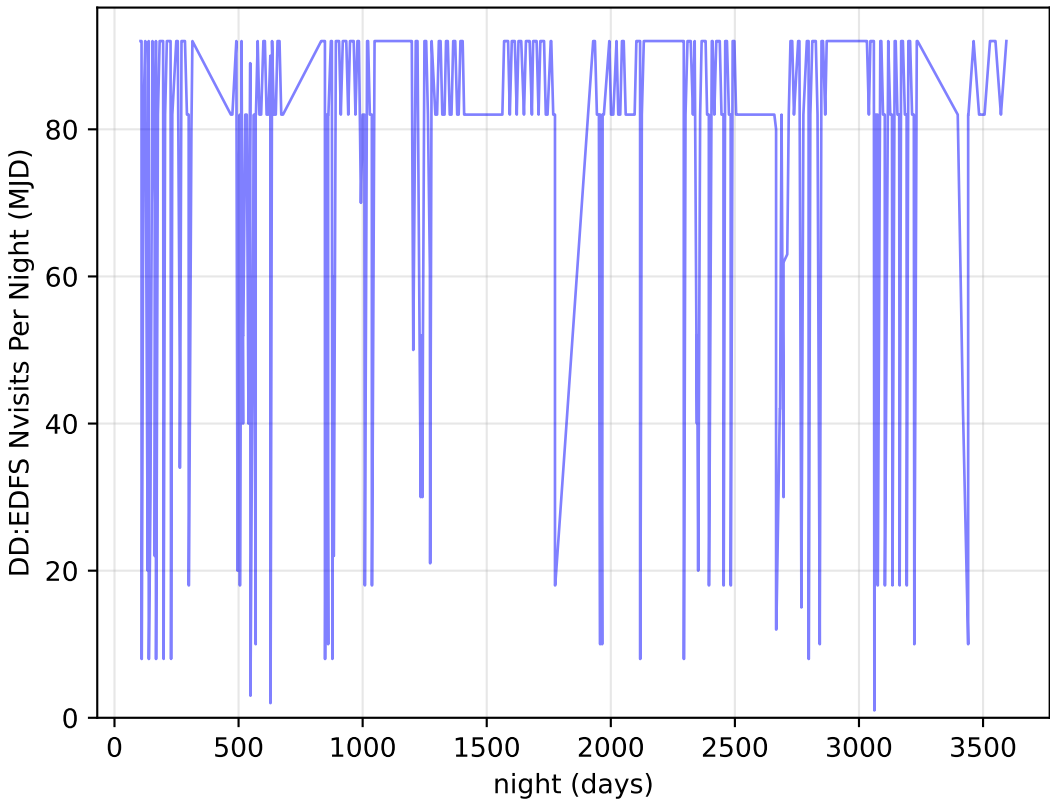
too_elab_r64_d3_griz_v3.4_10yrs all bands: DD:EDFS Nvisits Per Night
