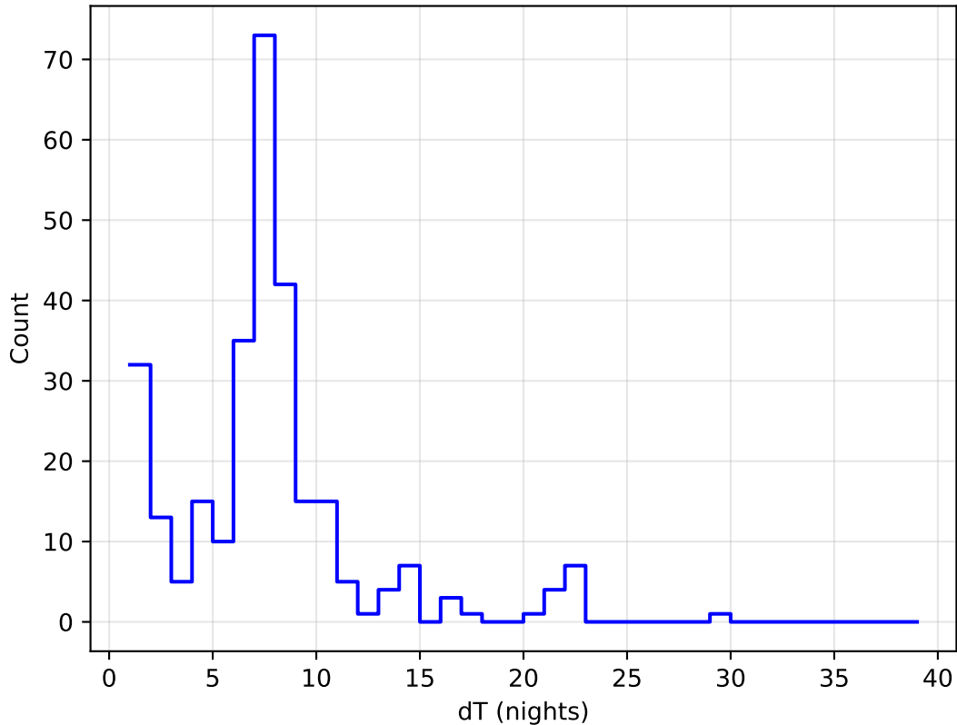
too_elab_r64_d3_griz_v3.4_10yrs all bands: DD:EDFS Delta Nights Histogram
