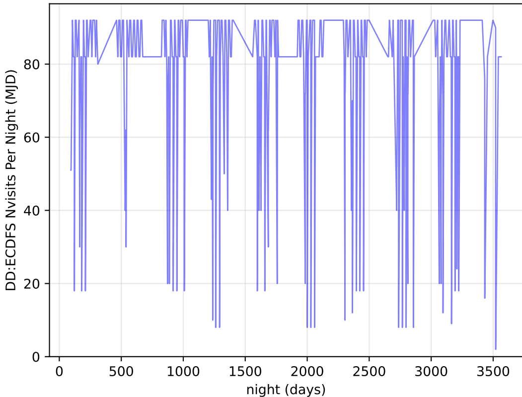
too_elab_r64_d3_griz_v3.4_10yrs all bands: DD:ECDFS Nvisits Per Night
