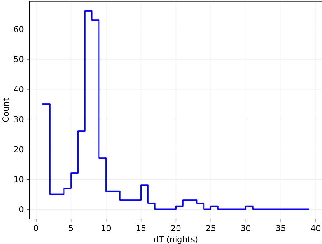
too_elab_r64_d3_griz_v3.4_10yrs all bands: DD:ECDFS Delta Nights Histogram
