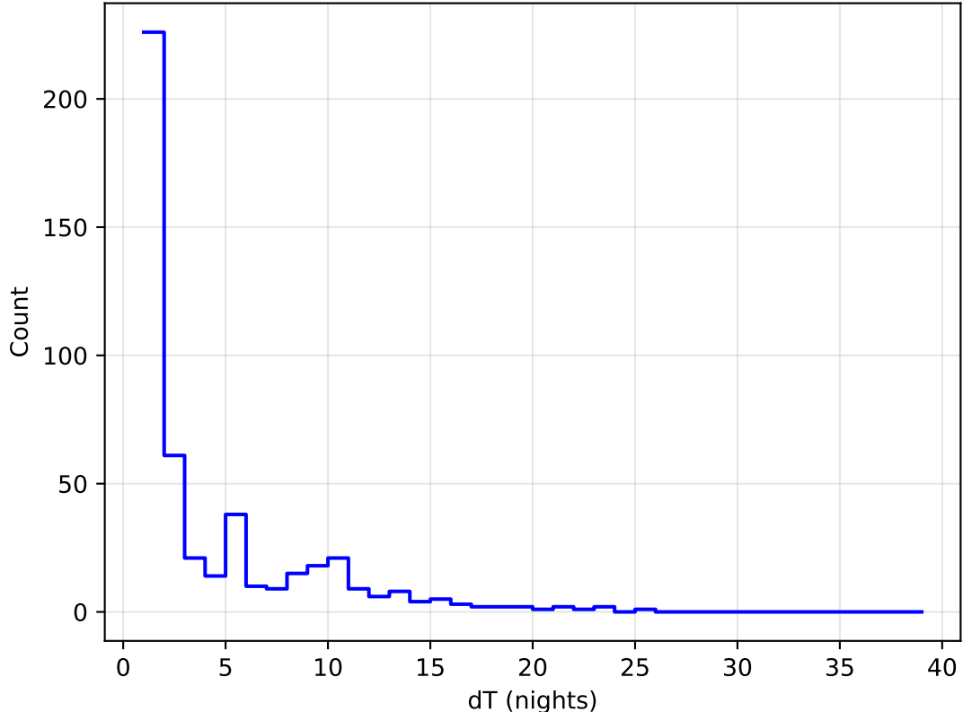
too_elab_r64_d3_griz_v3.4_10yrs all bands: DD: COSMOS Delta Nights Histogram
