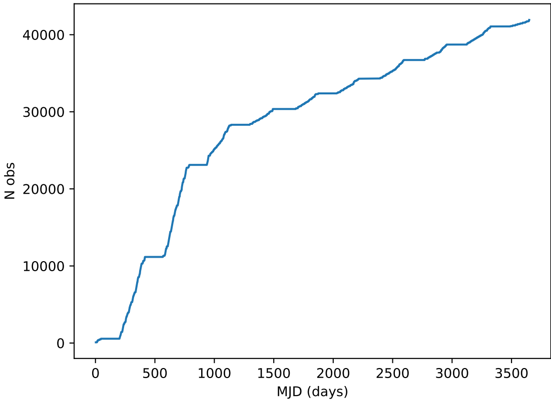
too_elab_r64_d3_griz_v3.4_10yrs all bands: DD: COSMOS Cumulative NVisits
