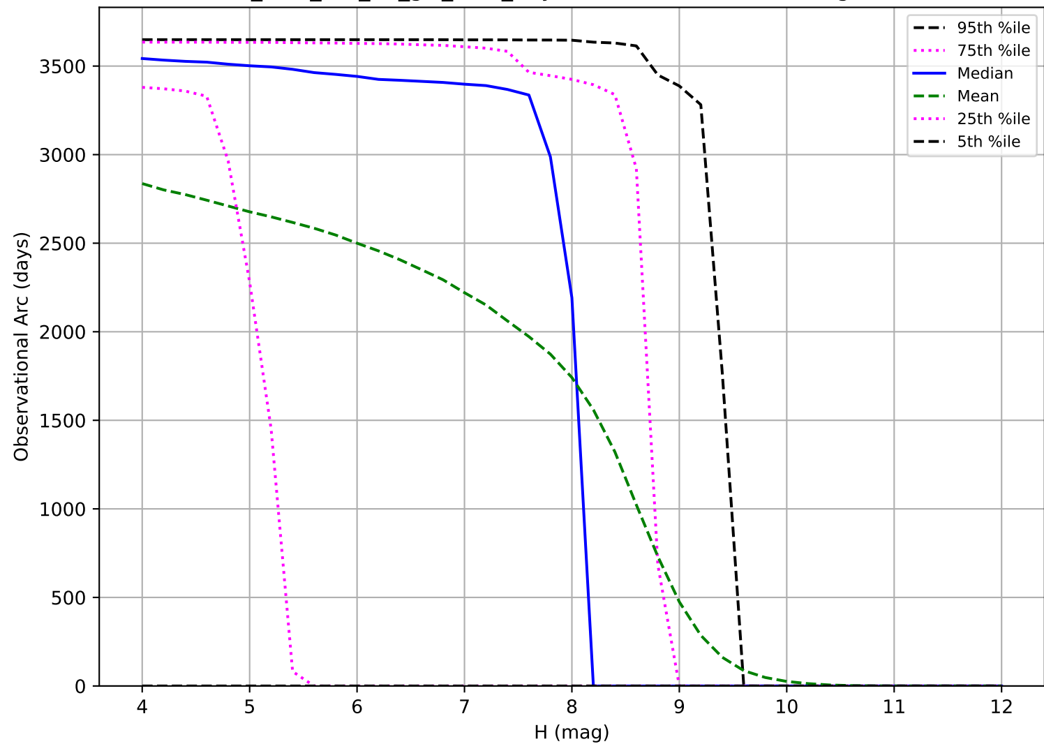
too_elab_r64_d3_giz_v3.4_10yrs: Observational Arc Length TNO
