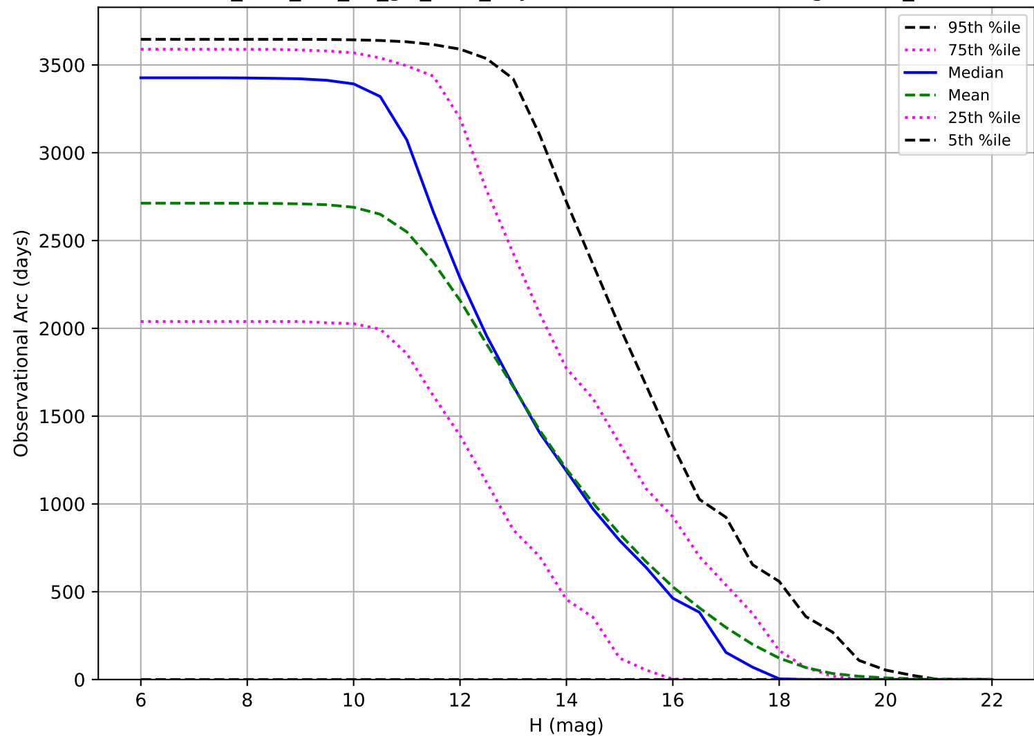
too_elab_r64_d3_giz_v3.4_10yrs: Observational Arc Length OCC_r5
