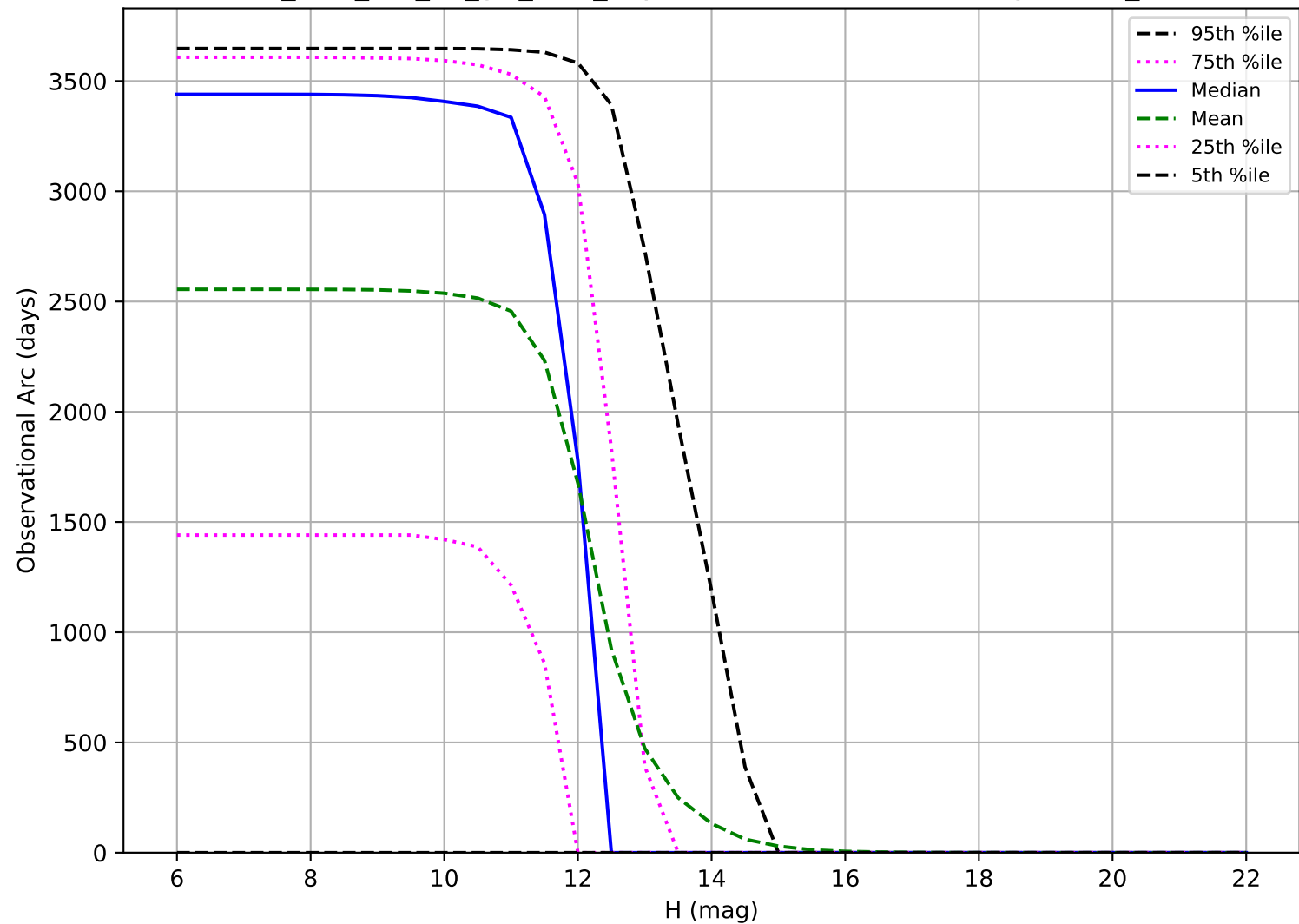
too_elab_r64_d3_giz_v3.4_10yrs: Observational Arc Length OCC_r20
