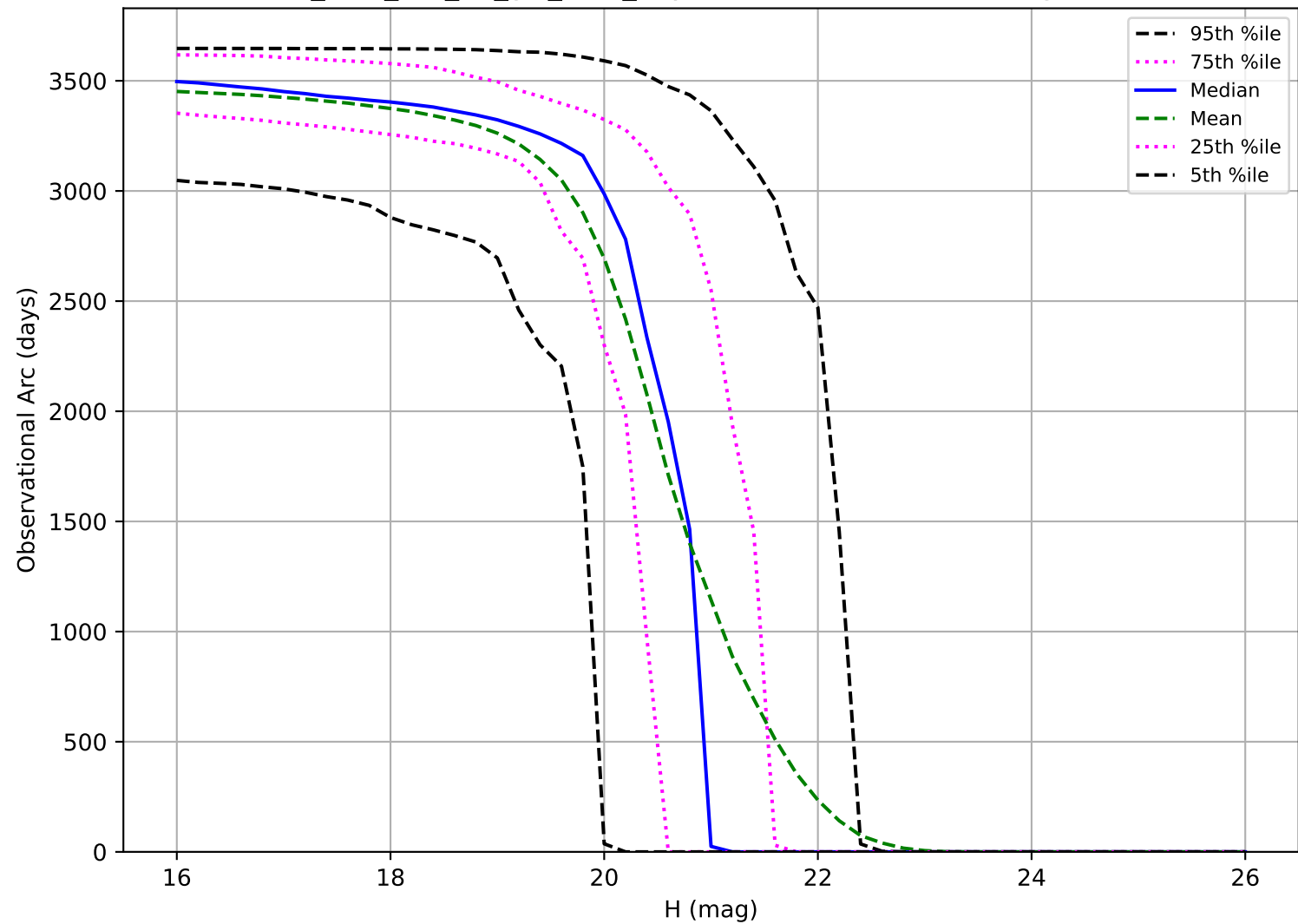
too_elab_r64_d3_giz_v3.4_10yrs: Observational Arc Length MBA
