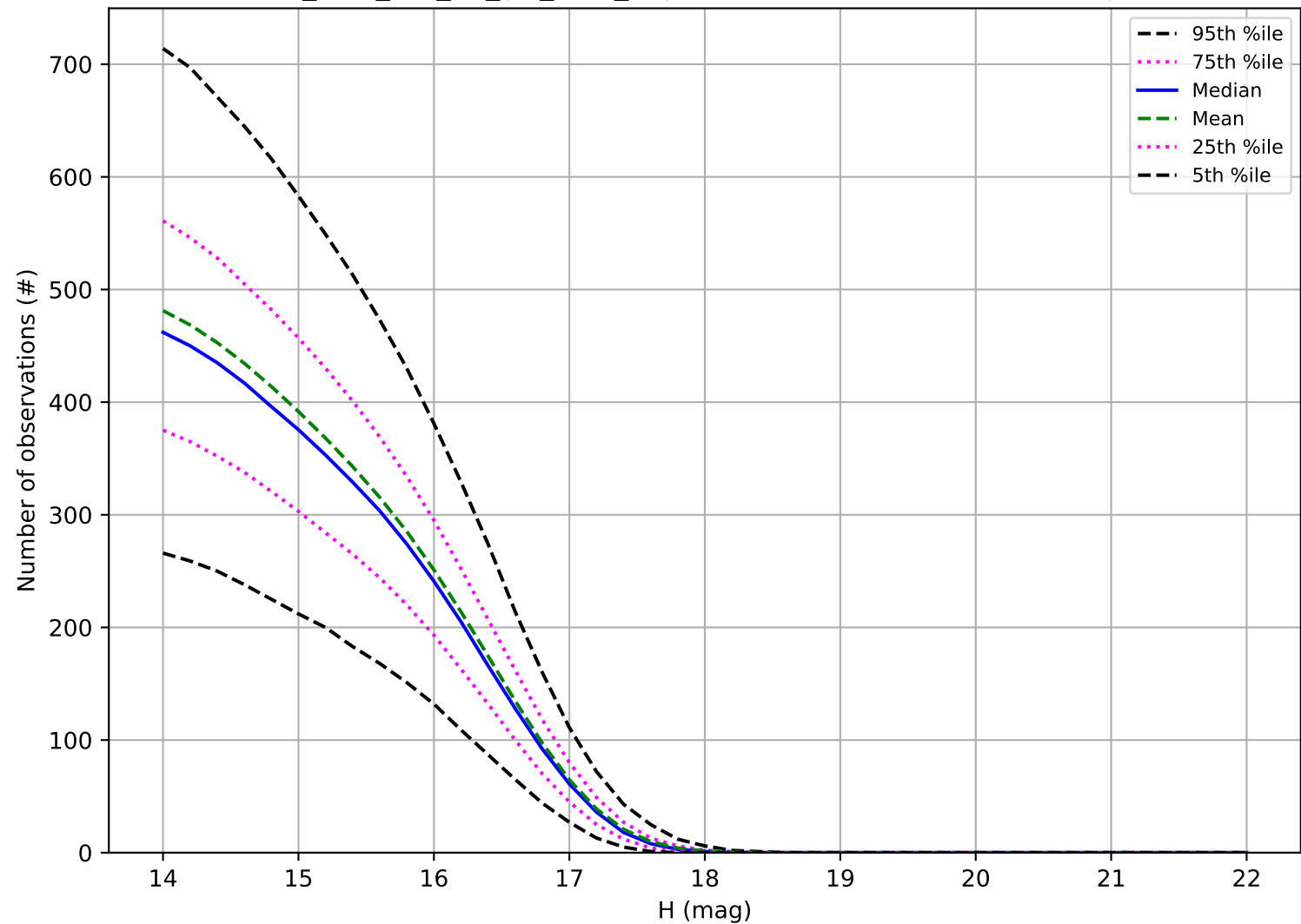
too_elab_r64_d3_giz_v3.4_10yrs: Number of observations Trojan
