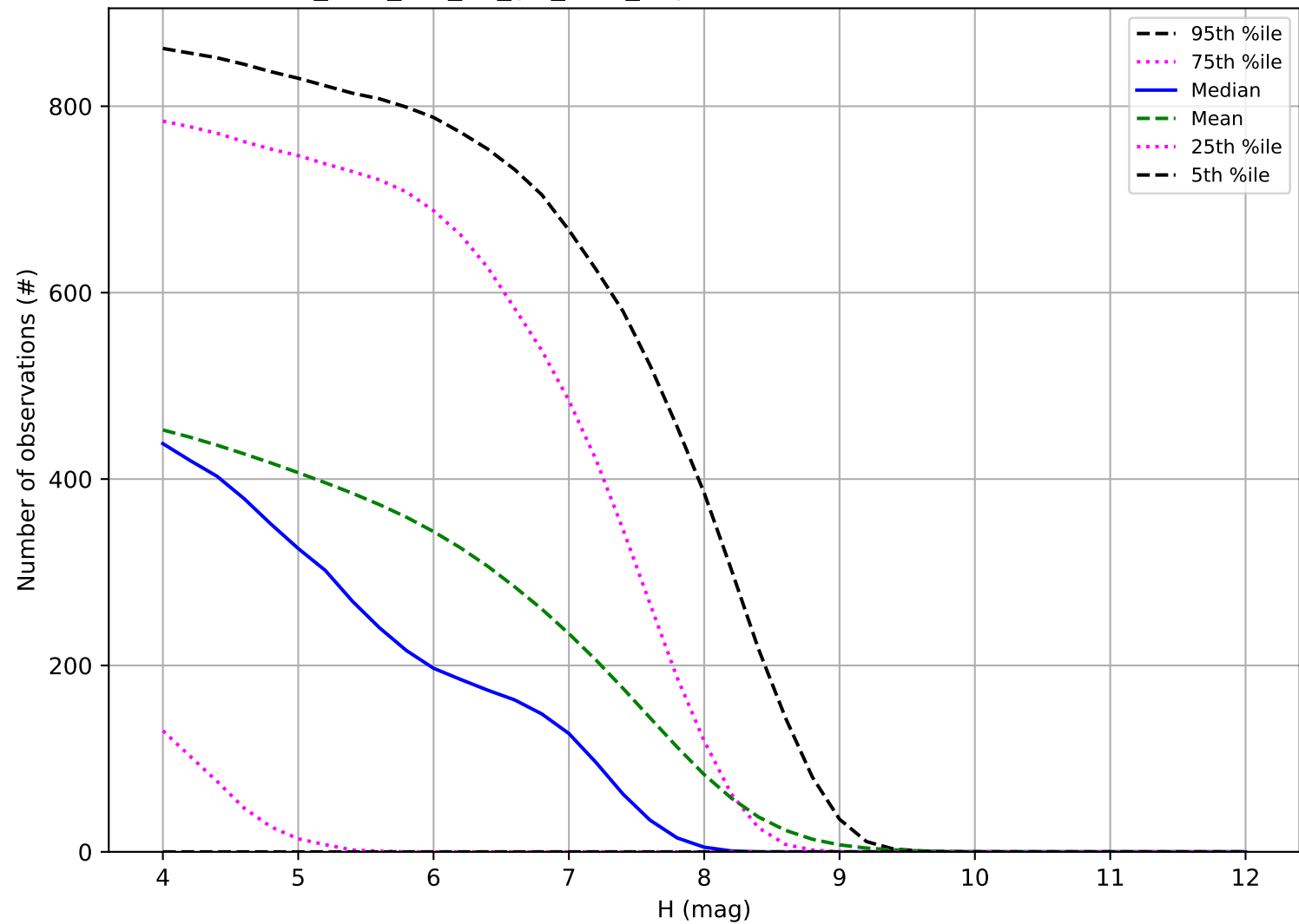
too_elab_r64_d3_giz_v3.4_10yrs: Number of observations TNO
