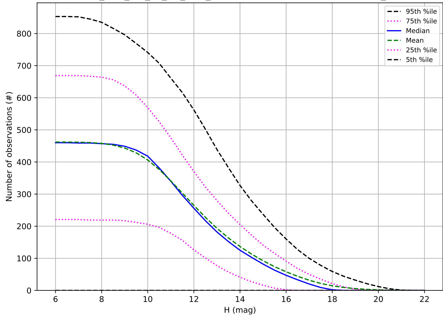
too_elab_r64_d3_giz_v3.4_10yrs: Number of observations OCC_r5
