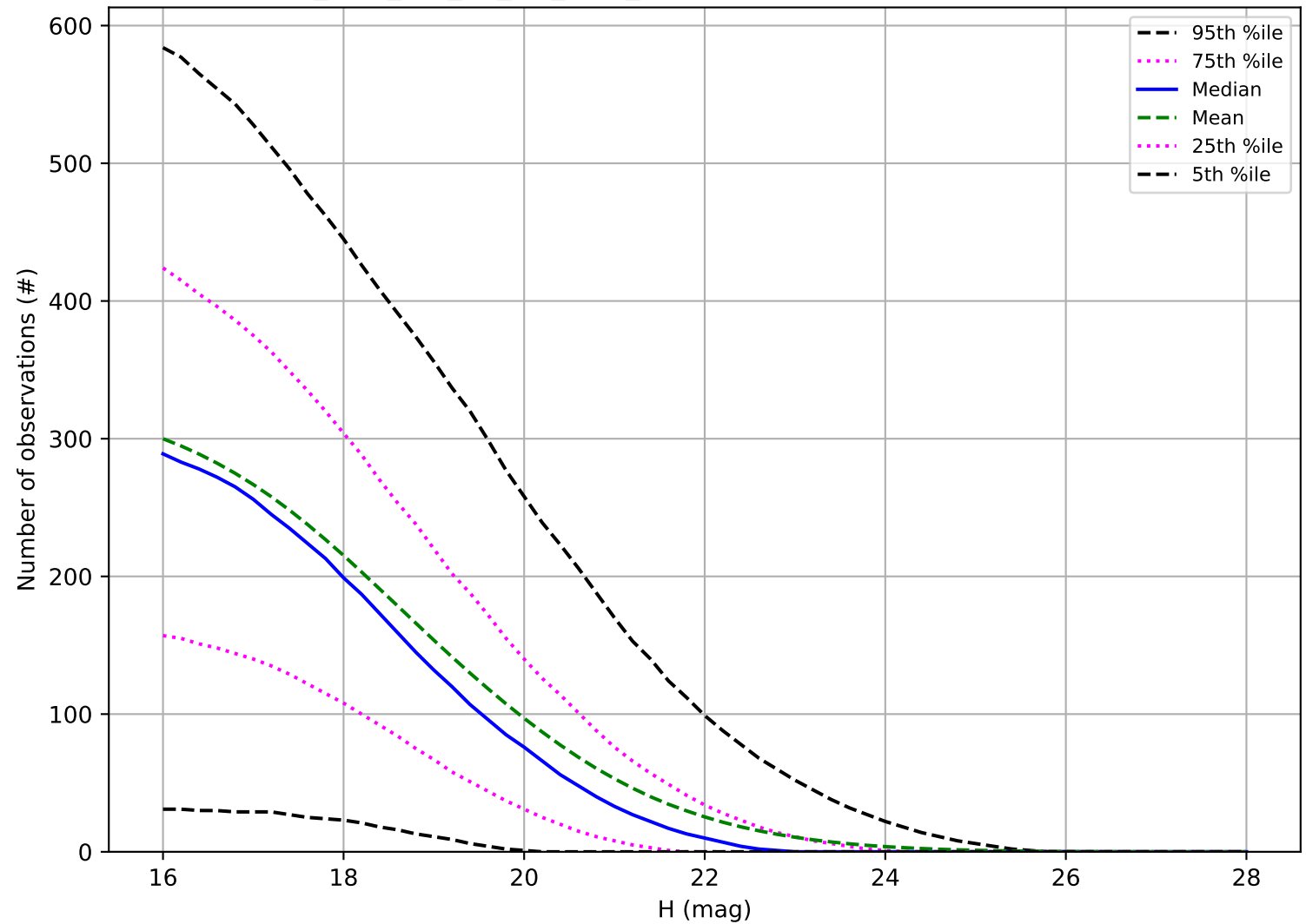
too_elab_r64_d3_giz_v3.4_10yrs: Number of observations NEO
