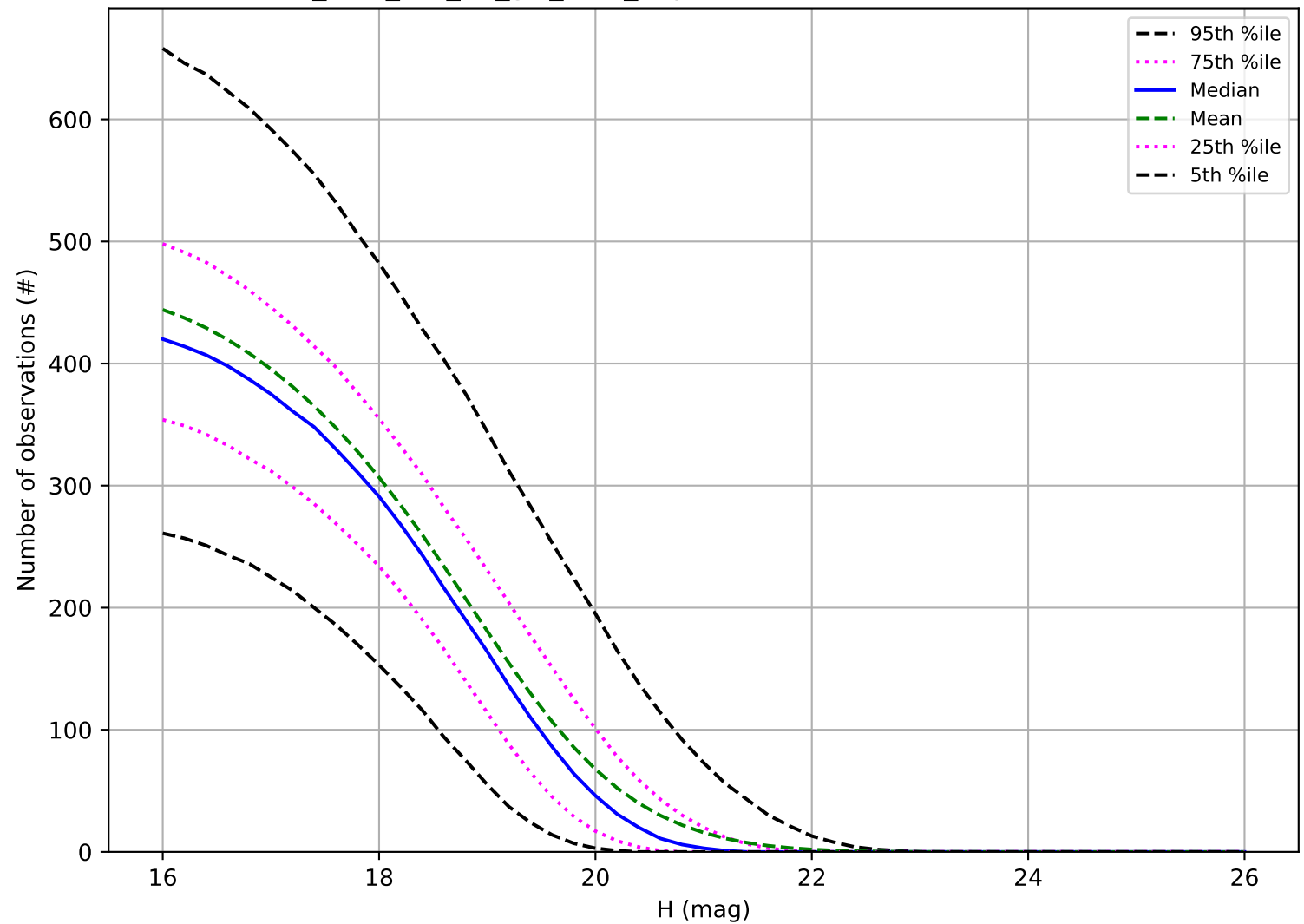
too_elab_r64_d3_giz_v3.4_10yrs: Number of observations MBA
