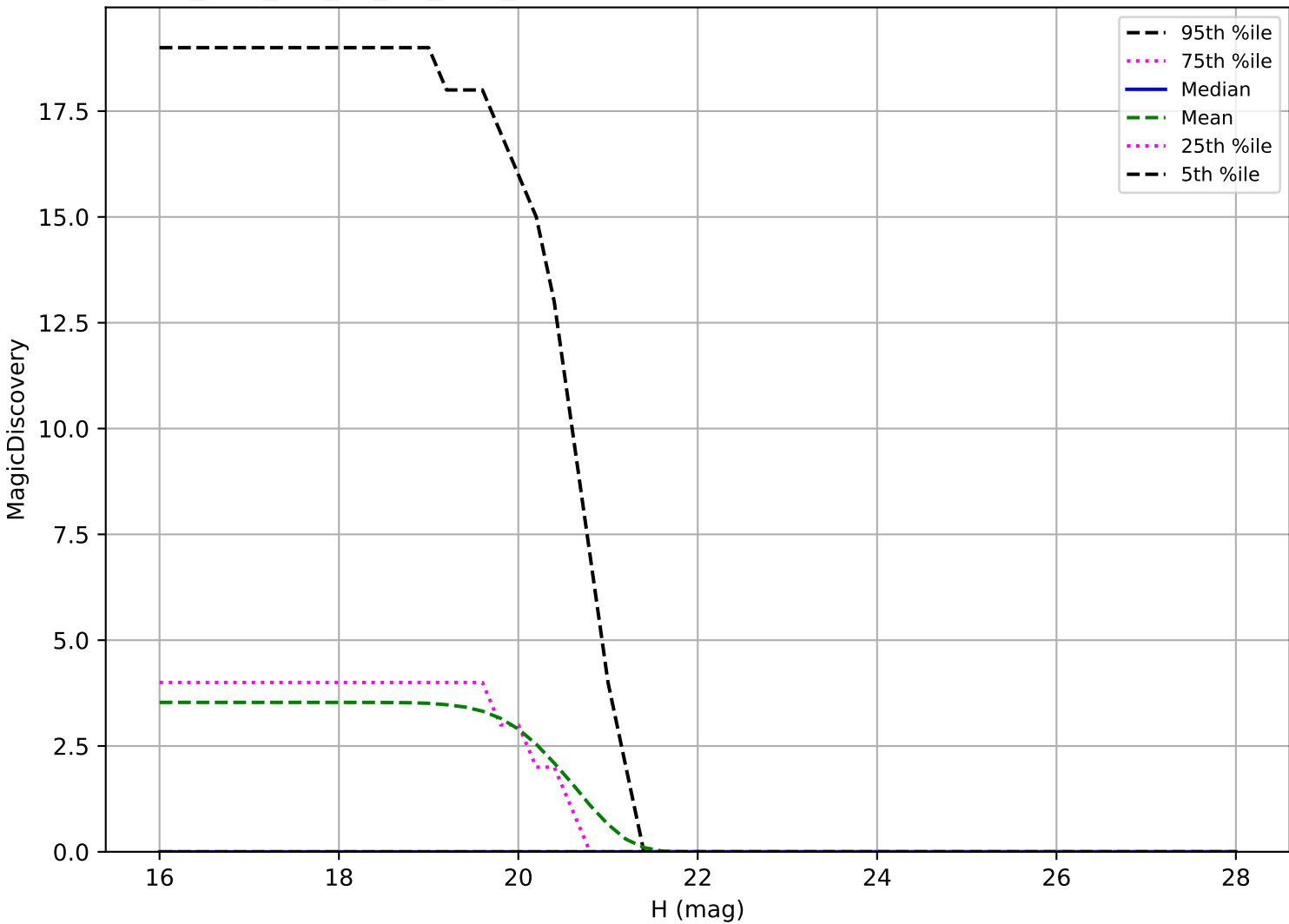
too_elab_r64_d3_giz_v3.4_10yrs: Vatira 6 detections in 60 nights detection loss
