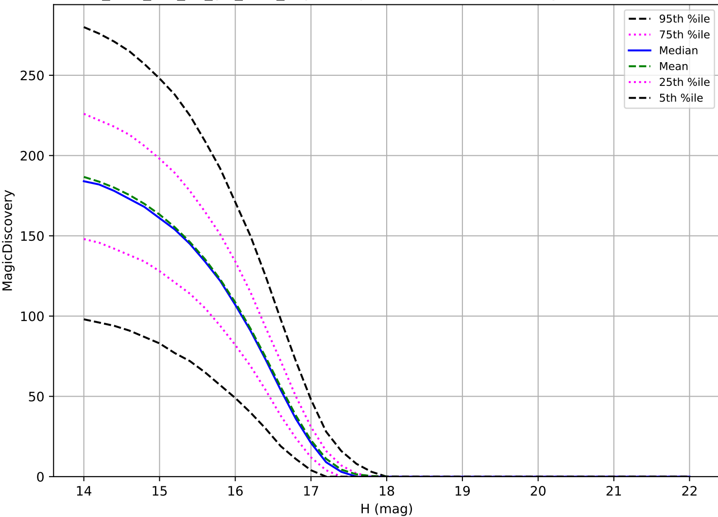
too_elab_r64_d3_giz_v3.4_10yrs: Trojan 6 detections in 60 nights detection loss
