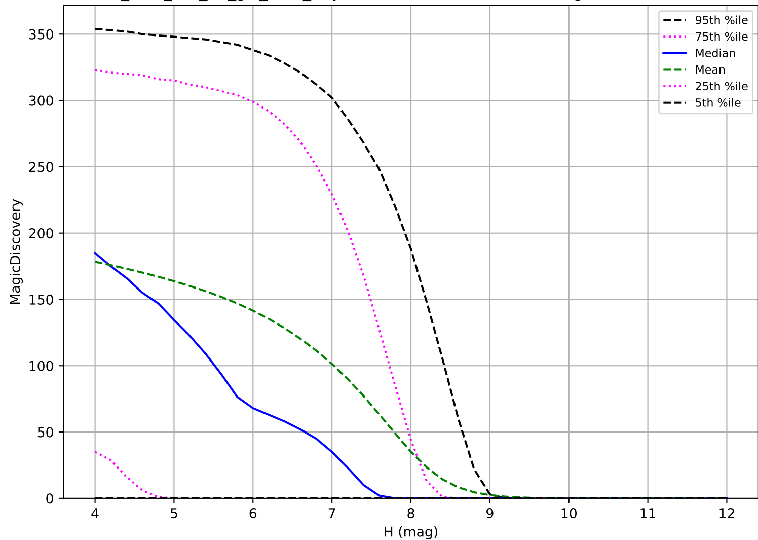
too_elab_r64_d3_giz_v3.4_10yrs: TNO 6 detections in 60 nights detection loss
