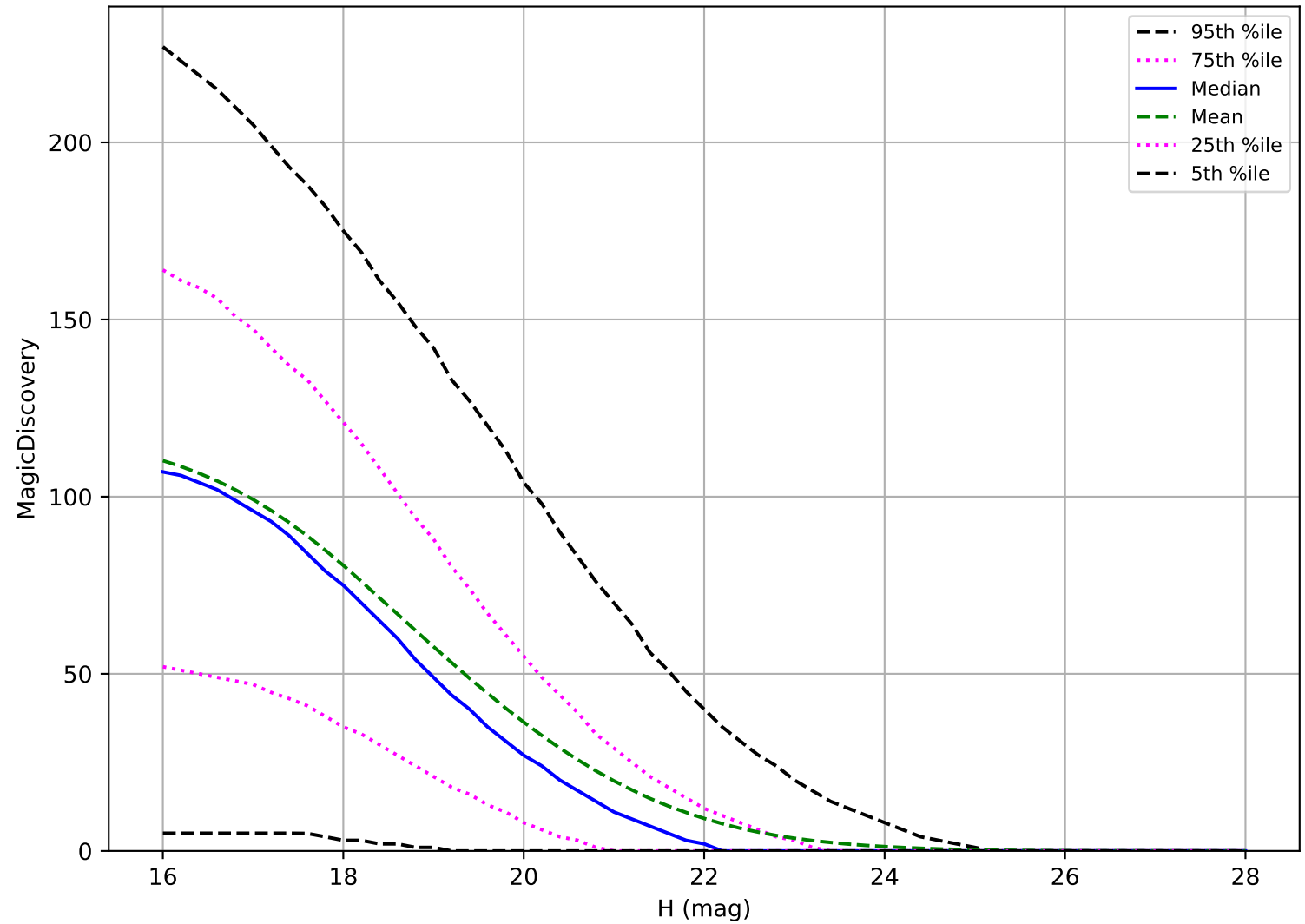
too_elab_r64_d3_giz_v3.4_10yrs: NEO 6 detections in 60 nights detection loss
