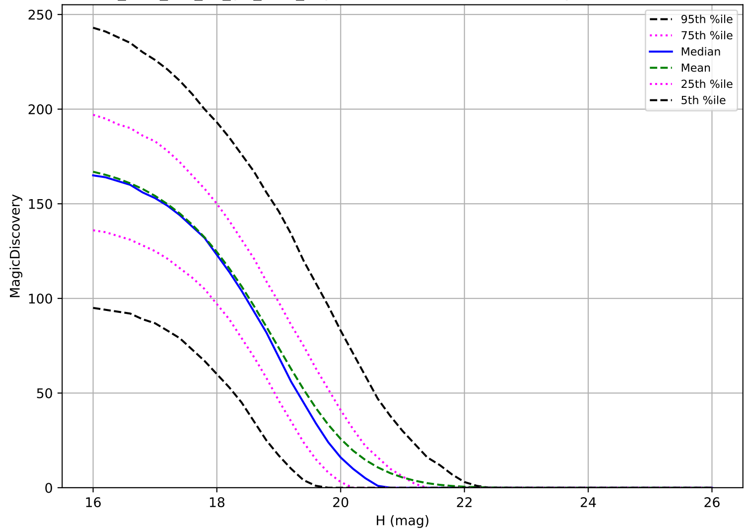
too_elab_r64_d3_giz_v3.4_10yrs: MBA 6 detections in 60 nights detection loss
