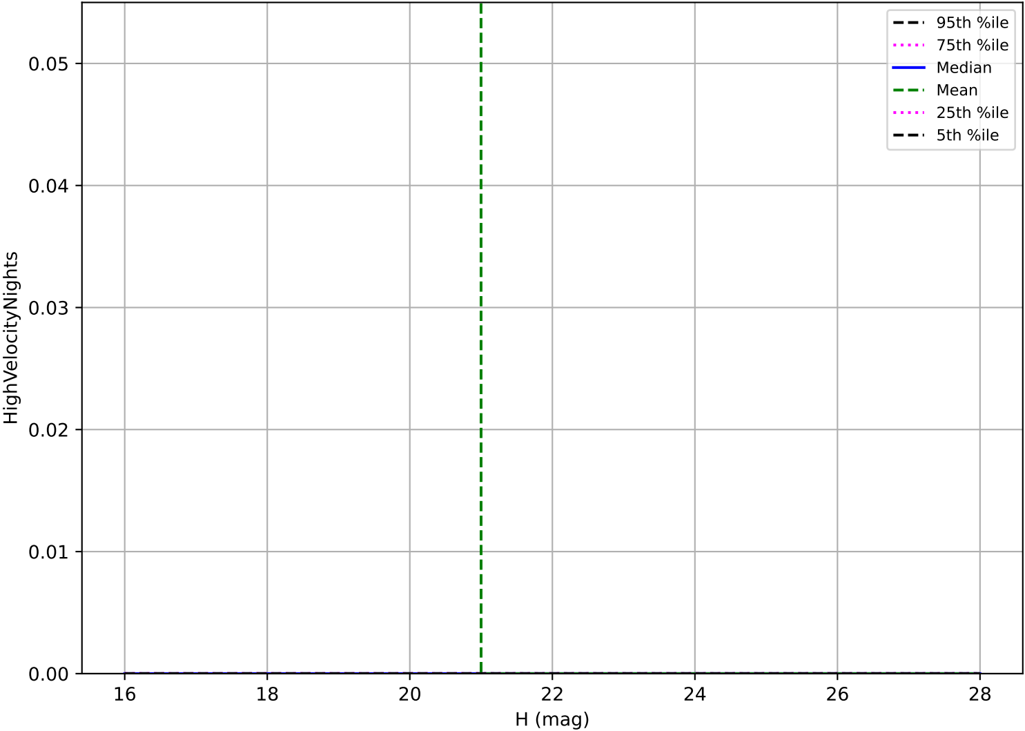
too_elab_r64_d3_giz_v3.4_10yrs: Vatira High velocity pair detection loss
