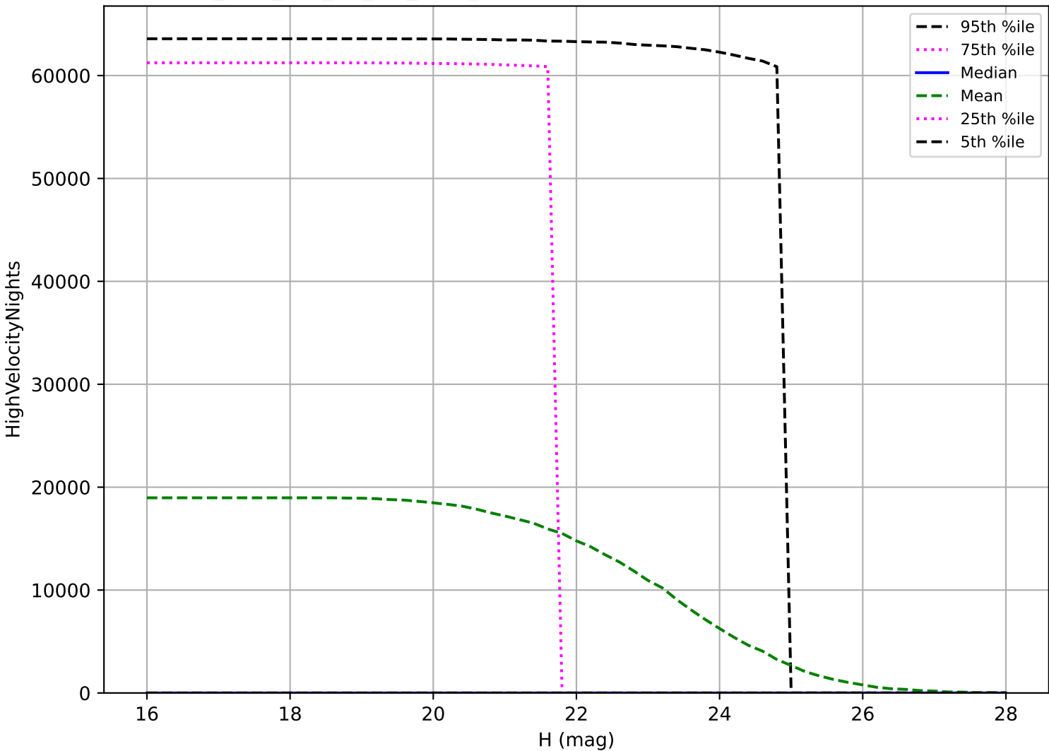
too_elab_r64_d3_giz_v3.4_10yrs: NEO High velocity pair detection loss
