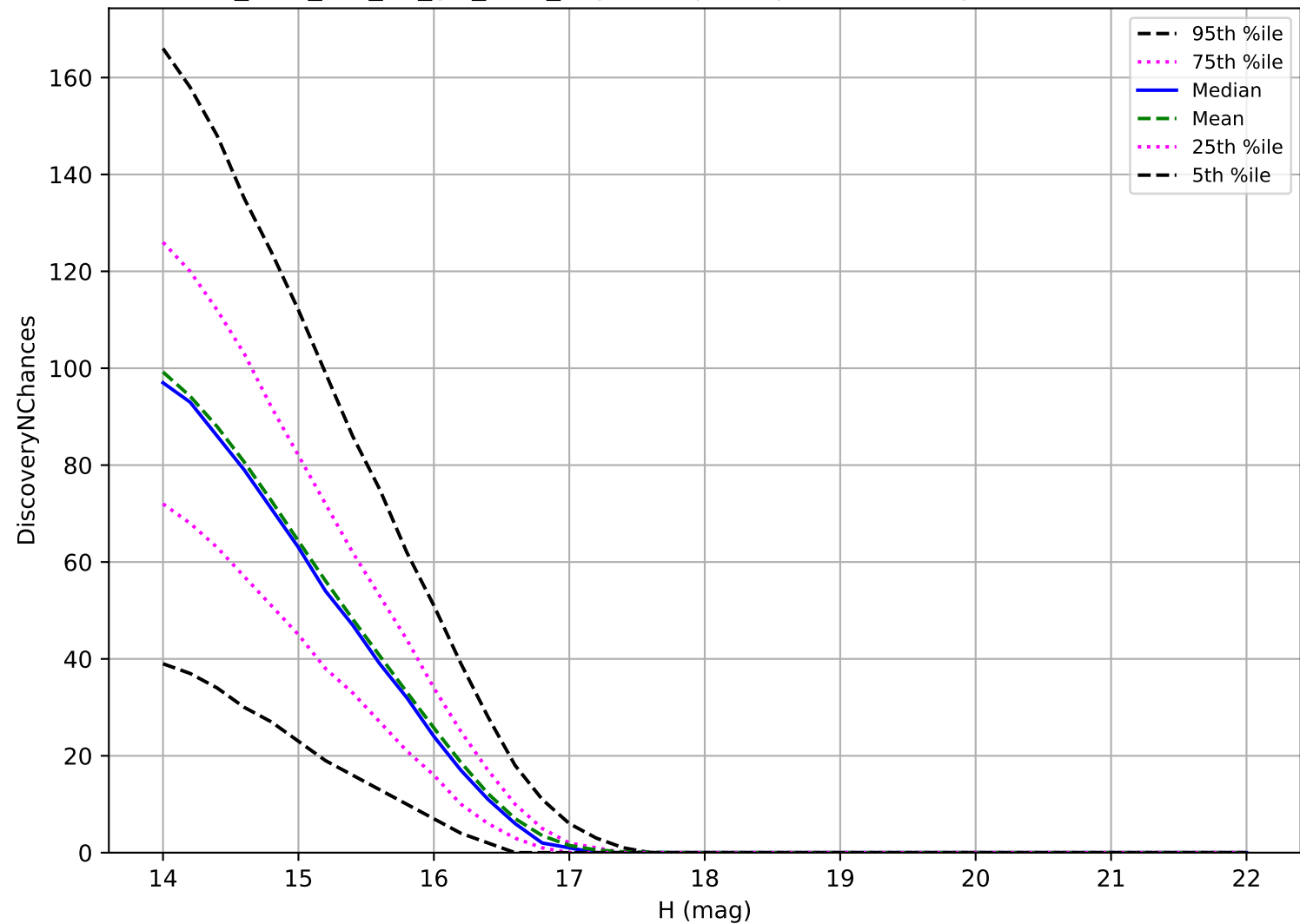
too_elab_r64_d3_giz_v3.4_10yrs: Trojan 3 pairs in 15 nights detection loss
