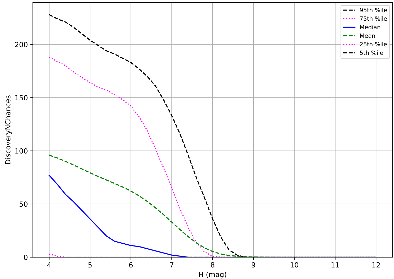
too_elab_r64_d3_giz_v3.4_10yrs: TNO 3 pairs in 15 nights detection loss
