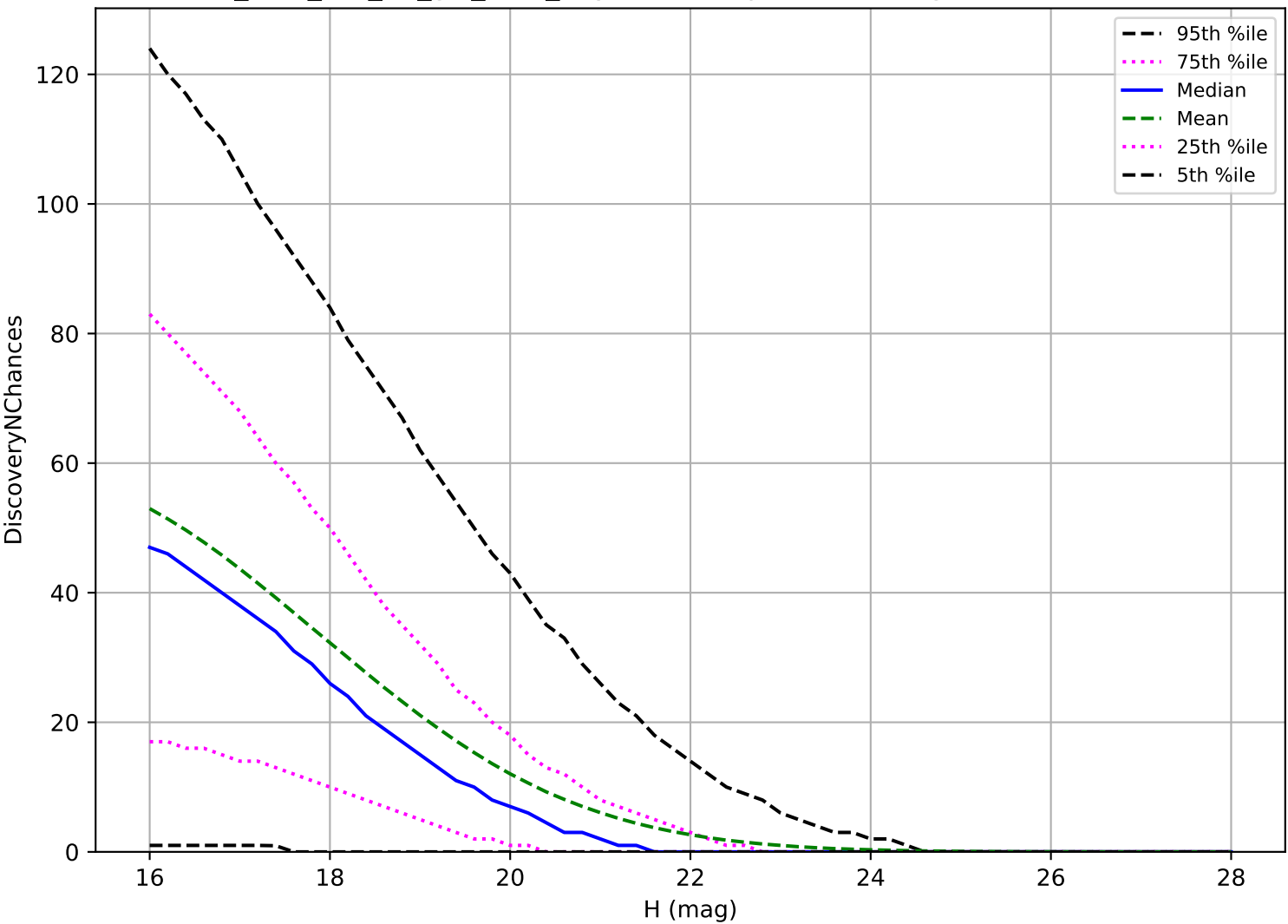
too_elab_r64_d3_giz_v3.4_10yrs: PHA 3 pairs in 15 nights detection loss
