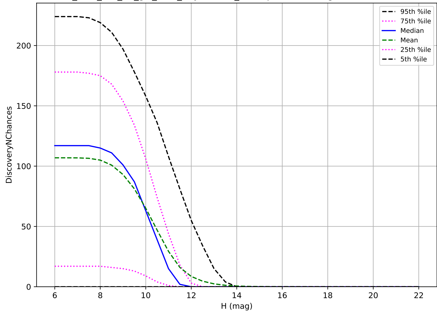
too_elab_r64_d3_giz_v3.4_10yrs: OCC_r20 3 pairs in 15 nights detection loss
