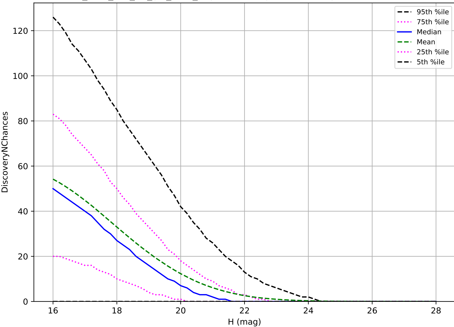
too_elab_r64_d3_giz_v3.4_10yrs: NEO 3 pairs in 15 nights detection loss
