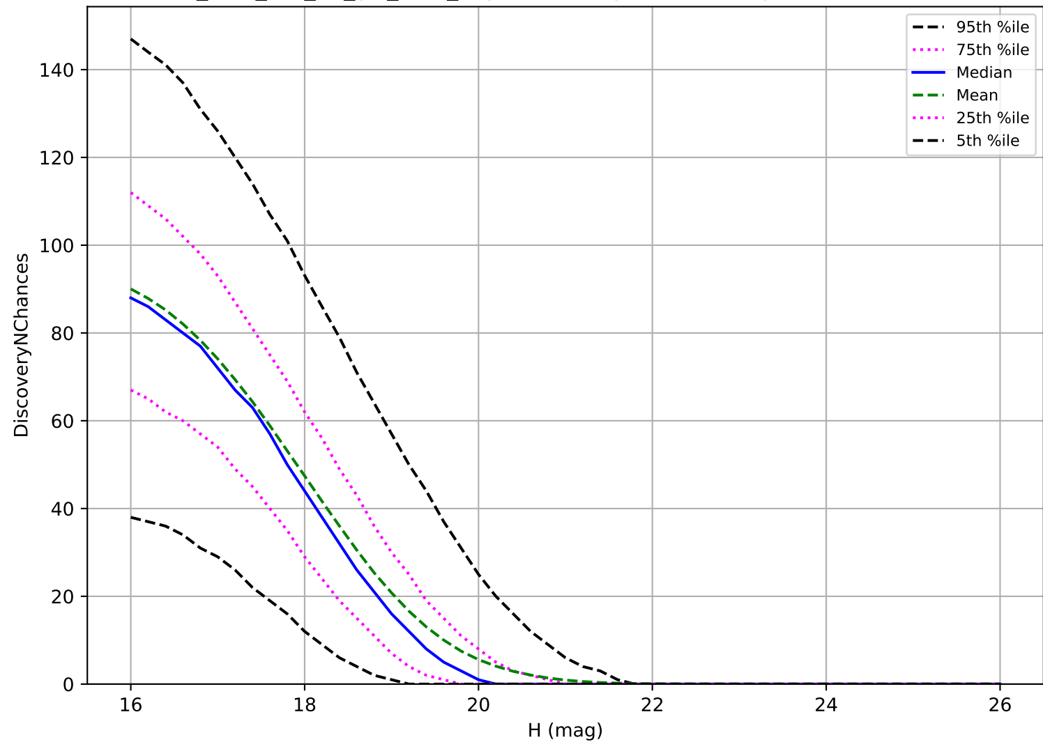
too_elab_r64_d3_giz_v3.4_10yrs: MBA 3 pairs in 15 nights detection loss
