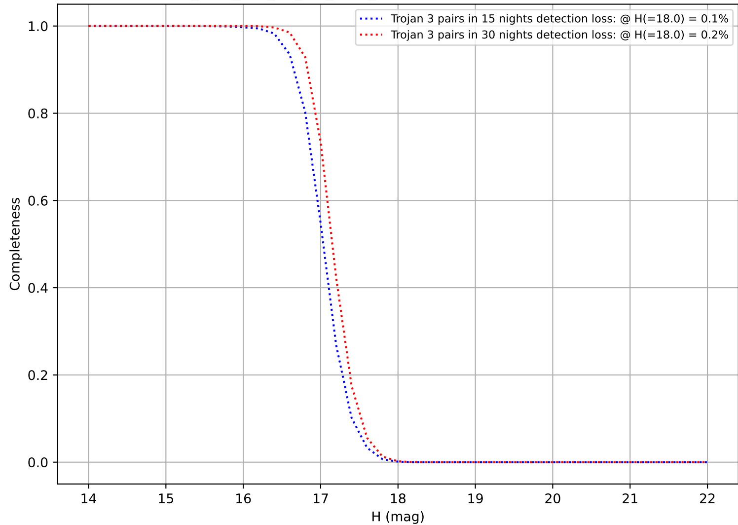
too_elab_r64_d3_giz_v3.4_10yrs: DifferentialCompleteness
