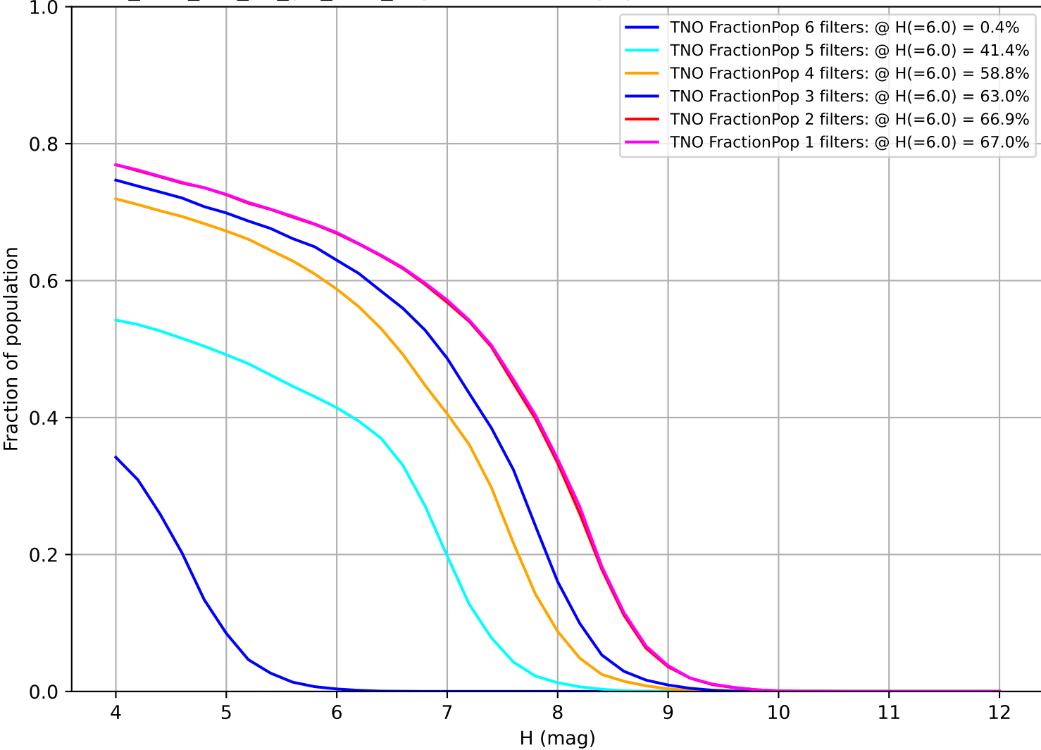
too_elab_r64_d3_giz_v3.4_10yrs: Fraction of population with colors in X filters TNO
