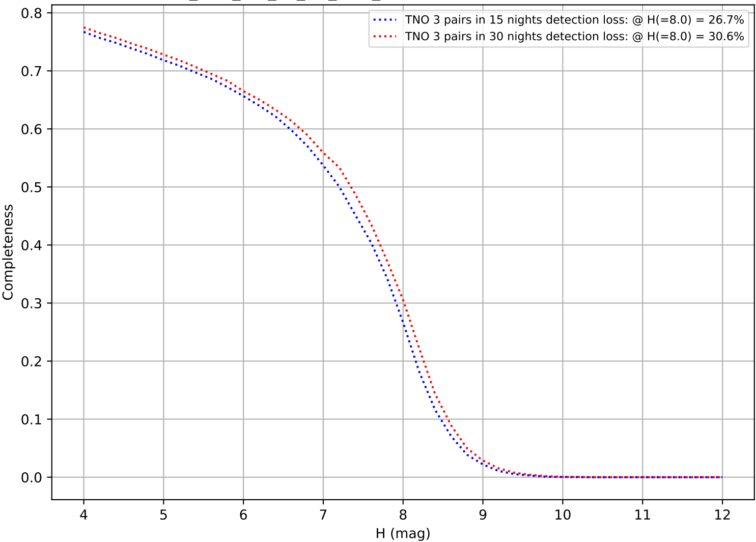
too_elab_r64_d3_giz_v3.4_10yrs: DifferentialCompleteness
