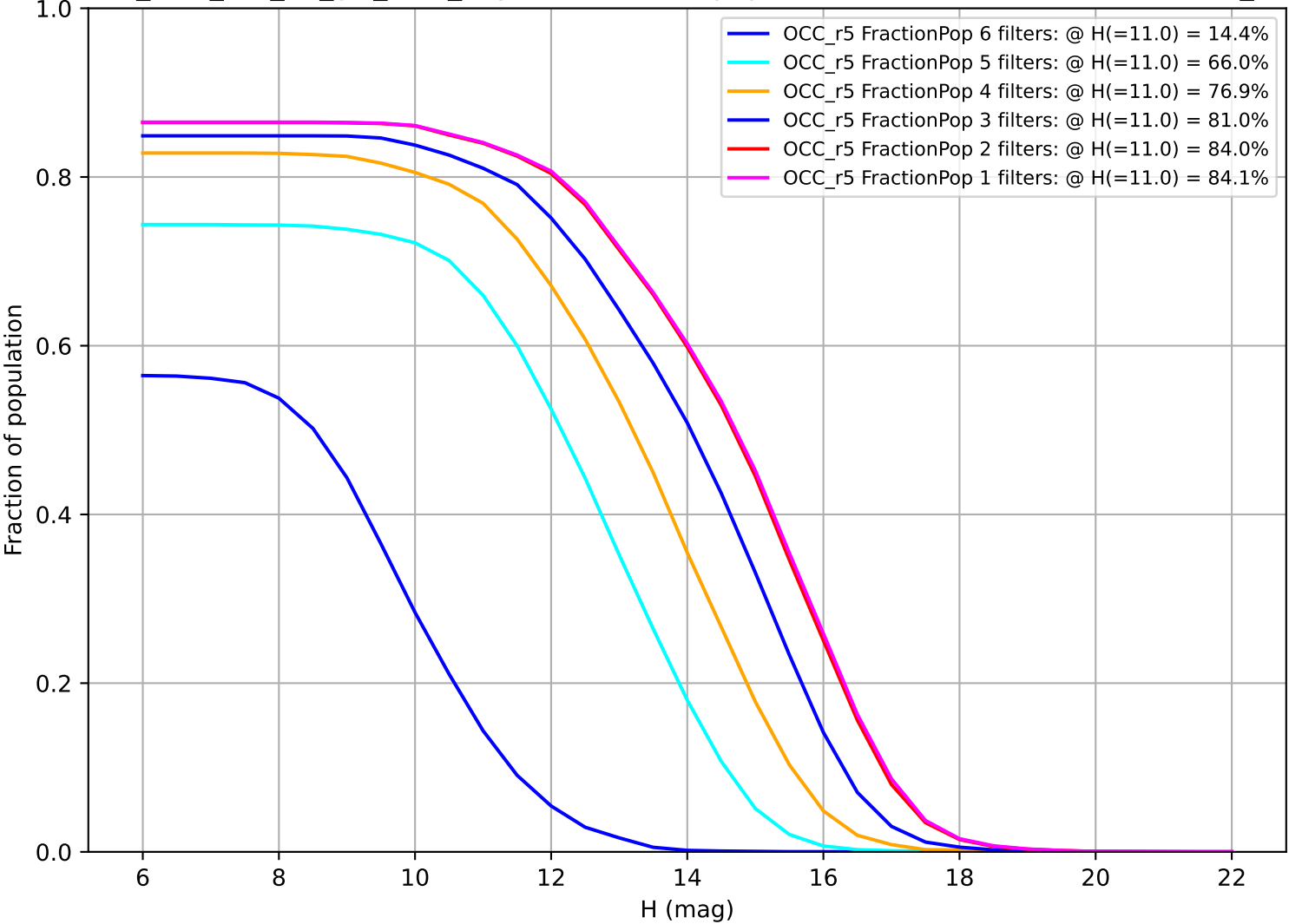
too_elab_r64_d3_giz_v3.4_10yrs: Fraction of population with colors in X filters OCC_r5
