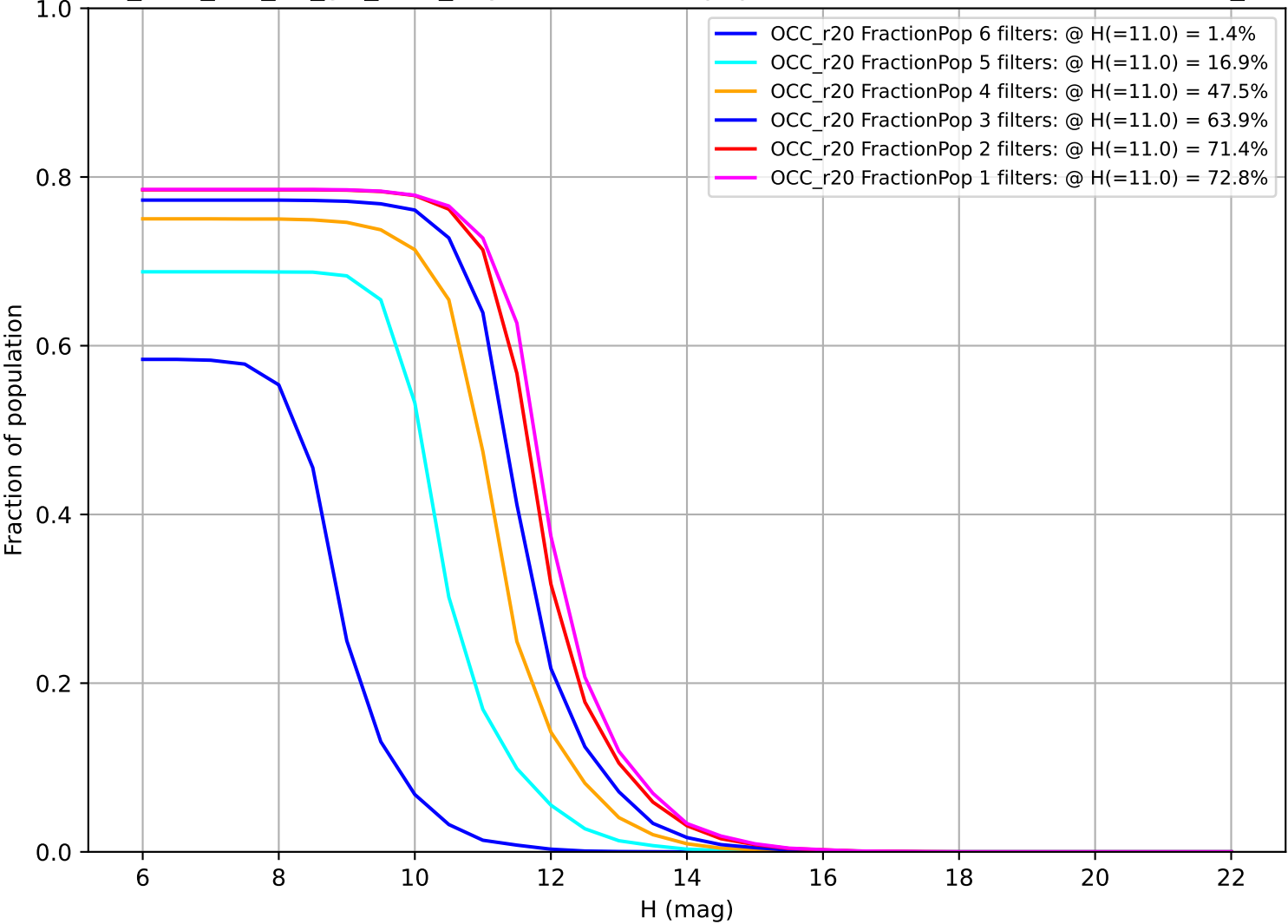
too_elab_r64_d3_giz_v3.4_10yrs: Fraction of population with colors in X filters OCC_r20
