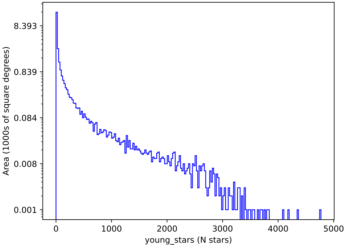
too_elab_r64_d3_giz_v3.4_10yrs : young_stars
