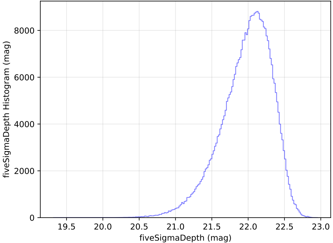
too_elab_r64_d3_giz_v3.4_10yrs y: fiveSigmaDepth Histogram
