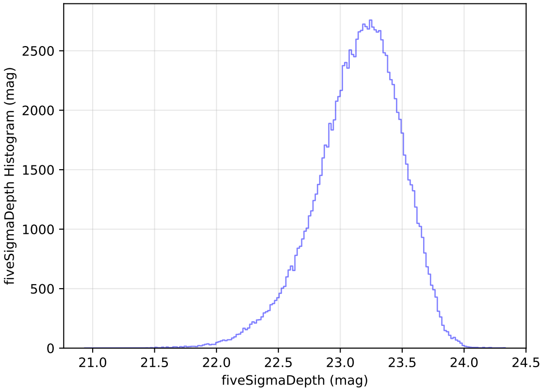
too_elab_r64_d3_giz_v3.4_10yrs u: fiveSigmaDepth Histogram
