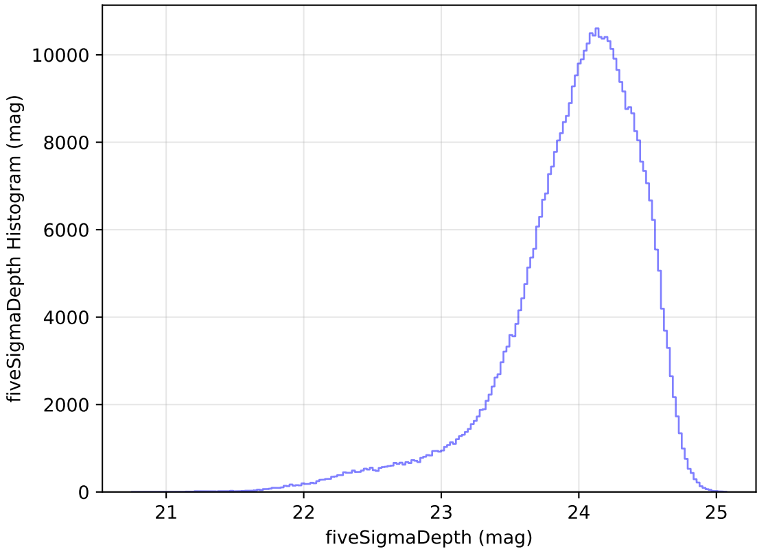
too_elab_r64_d3_giz_v3.4_10yrs r: fiveSigmaDepth Histogram
