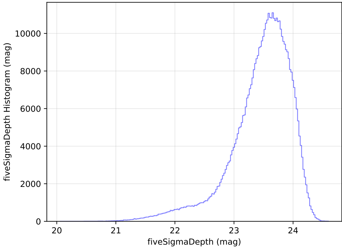
too_elab_r64_d3_giz_v3.4_10yrs i: fiveSigmaDepth Histogram
