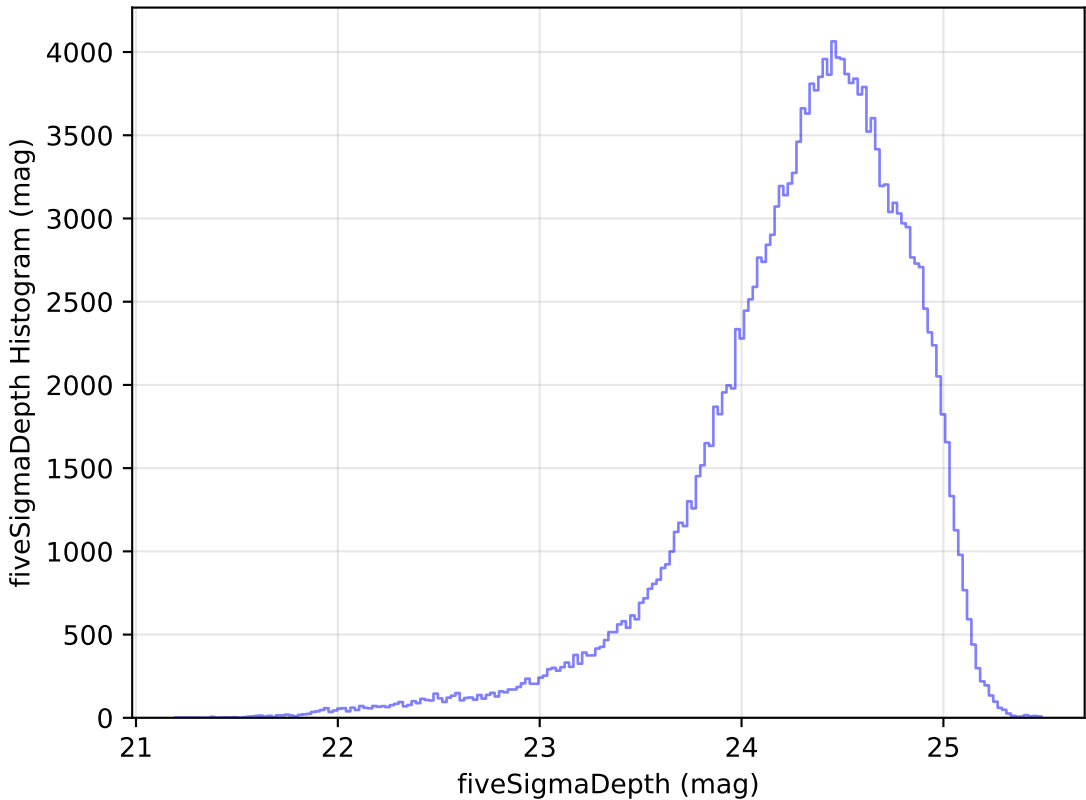
too_elab_r64_d3_giz_v3.4_10yrs g: fiveSigmaDepth Histogram
