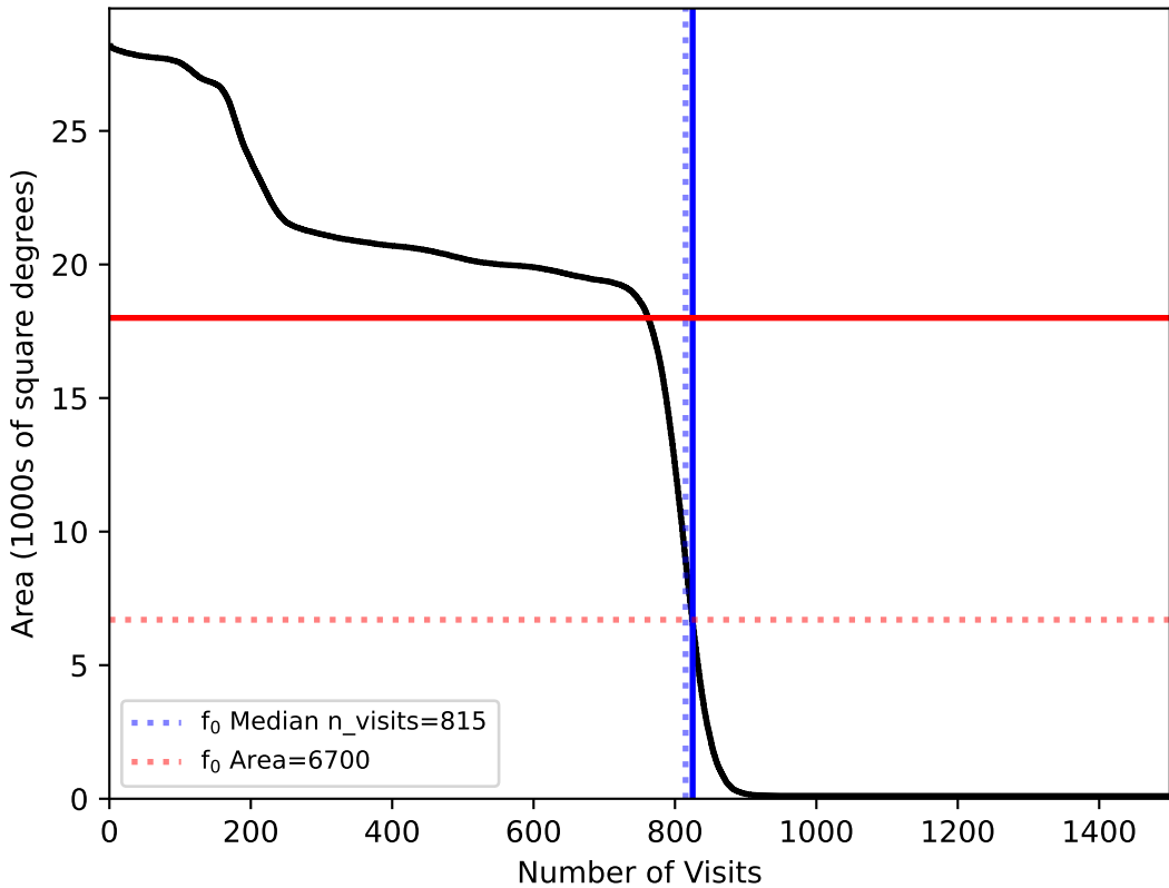
too_elab_r64_d3_giz_v3.4_10yrs : f0
