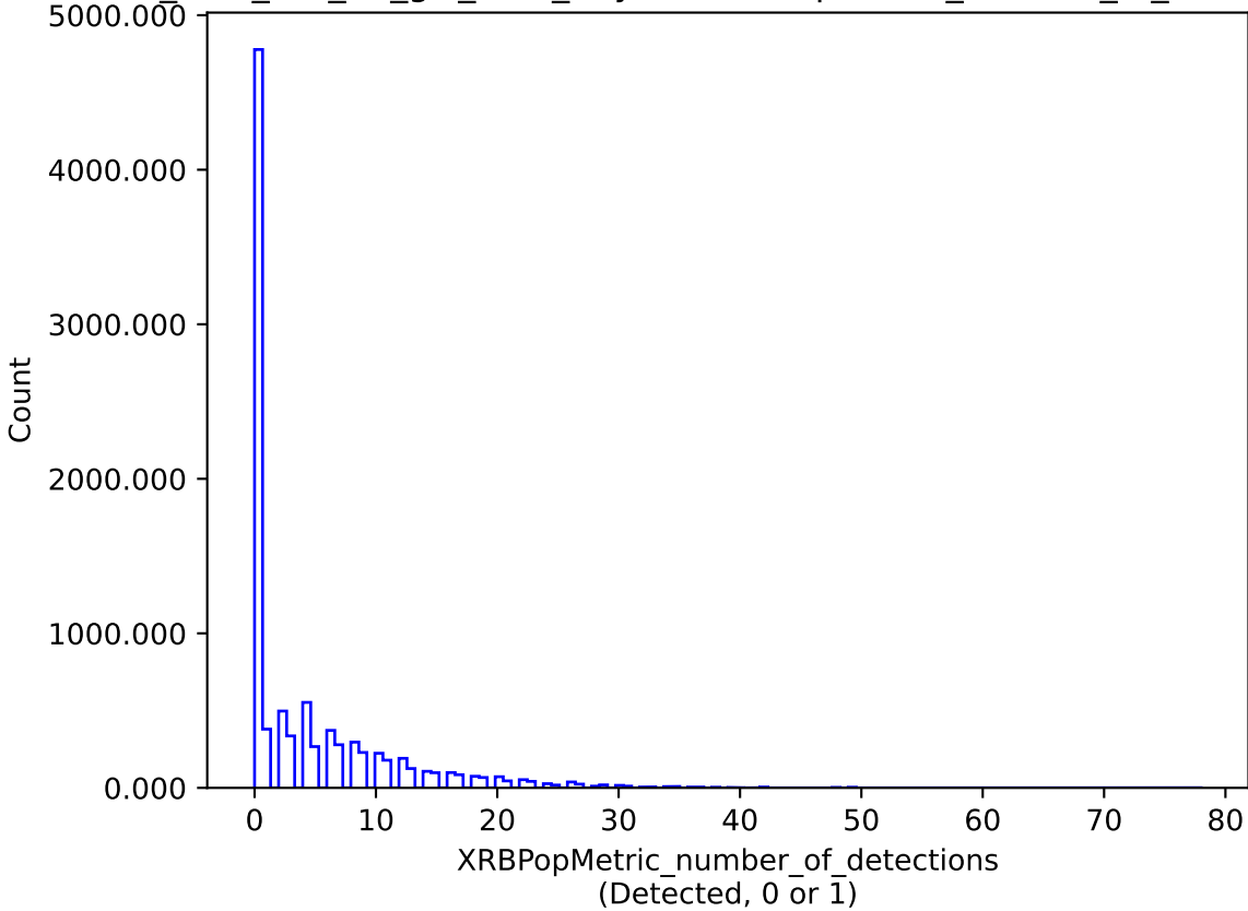
too_elab_r64_d3_giz_v3.4_10yrs : XRBPoMetric_number_of_detections
