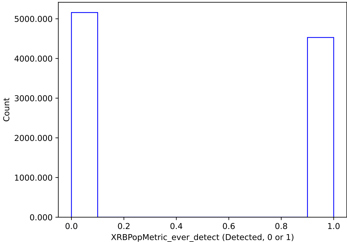
too_elab_r64_d3_giz_v3.4_10yrs : XRBPoMetric_ever_detect
