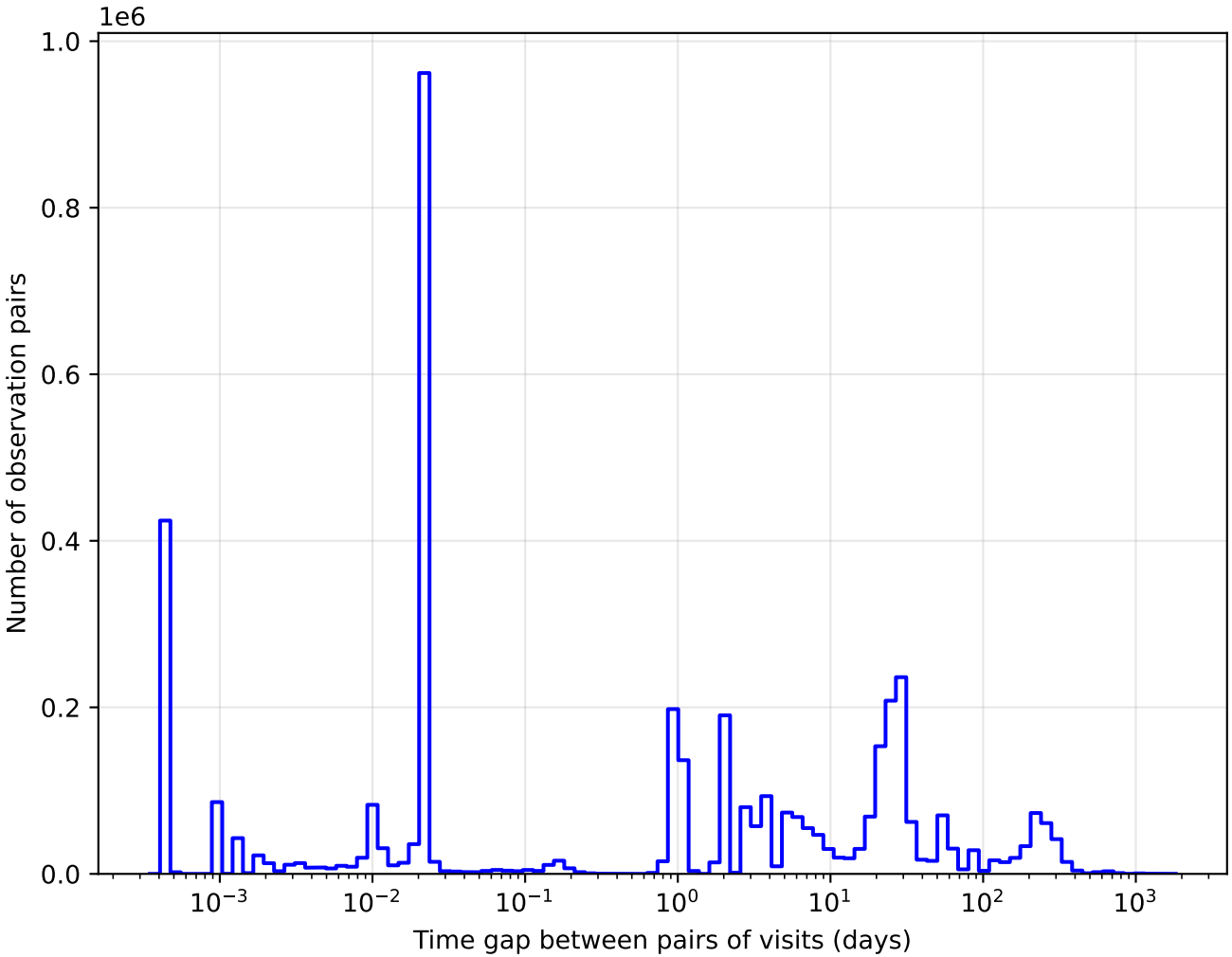
too_elab_r64_d3_giz_v3.4_10yrs y band: Tgaps observationStartMJD
