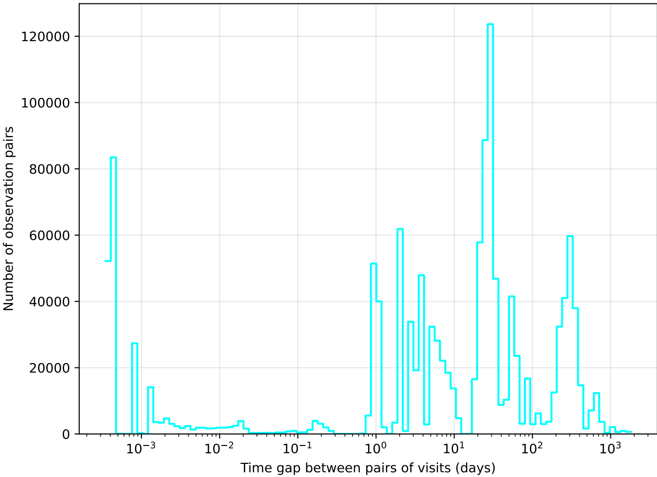
too_elab_r64_d3_giz_v3.4_10yrs u band: Tgaps observationStartMJD
