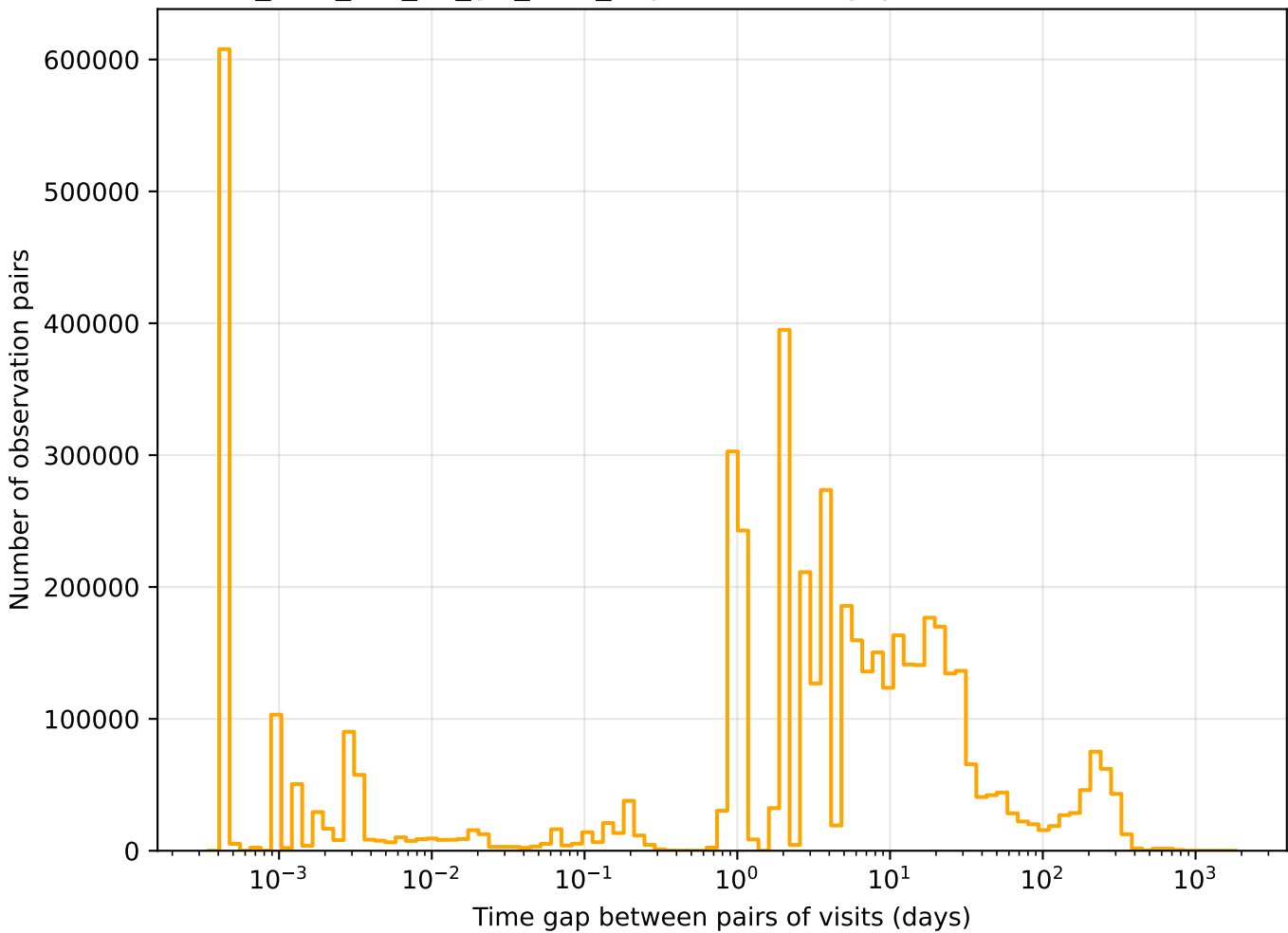
too_elab_r64_d3_giz_v3.4_10yrs r band: Tgaps observationStartMJD
