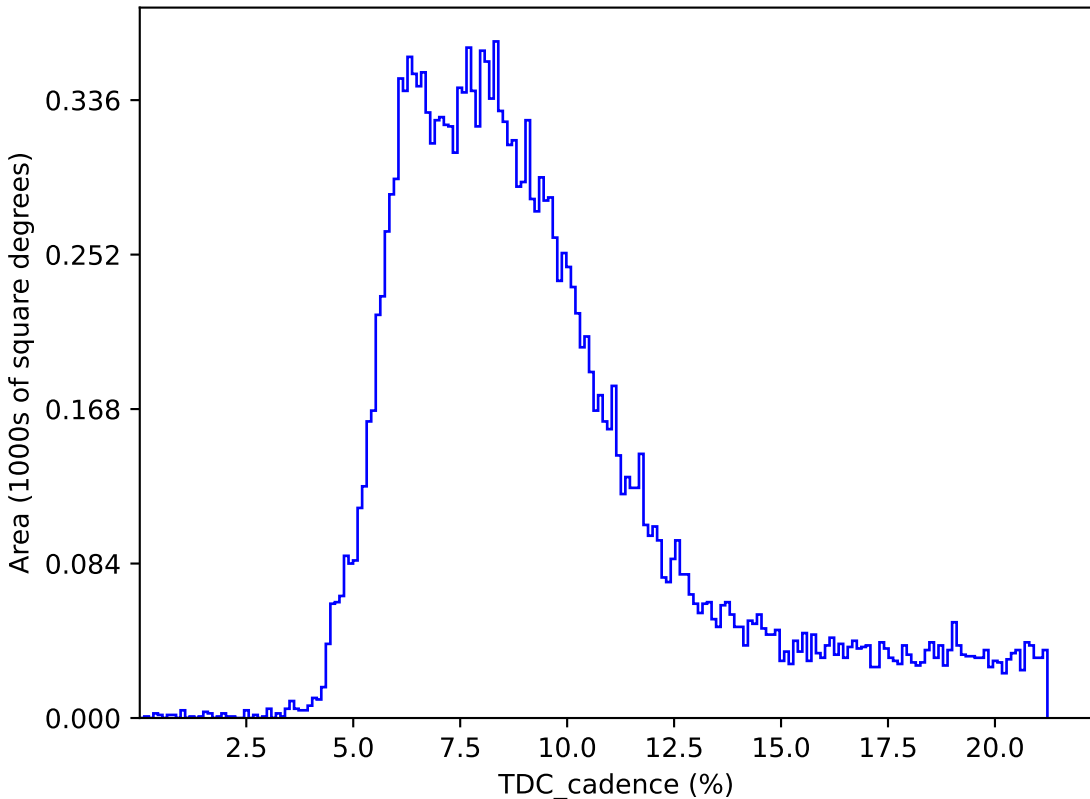
too_elab_r64_d3_giz_v3.4_10yrs : TDC_cadence
