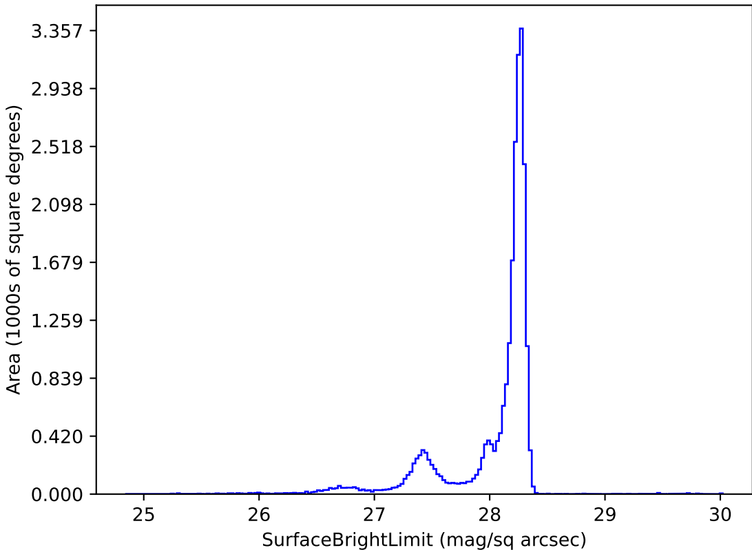
too_elab_r64_d3_giz_v3.4_10yrs y: SurfaceBrightLimit
