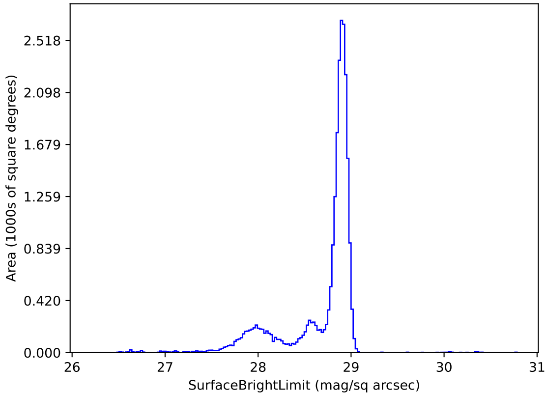
too_elab_r64_d3_giz_v3.4_10yrs u: SurfaceBrightLimit
